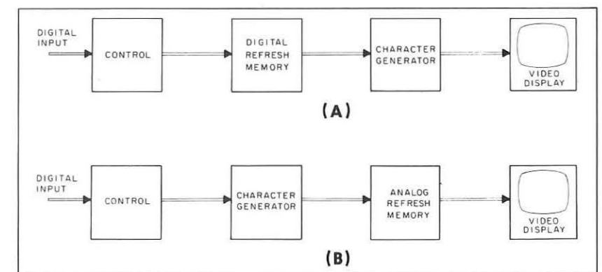
Figure 1. Raster scan CRT displays
