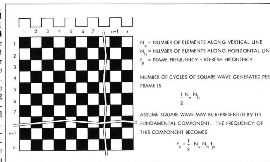
Figure 1. Checker Board Pattern — An Estimate of System Bandwidth.
